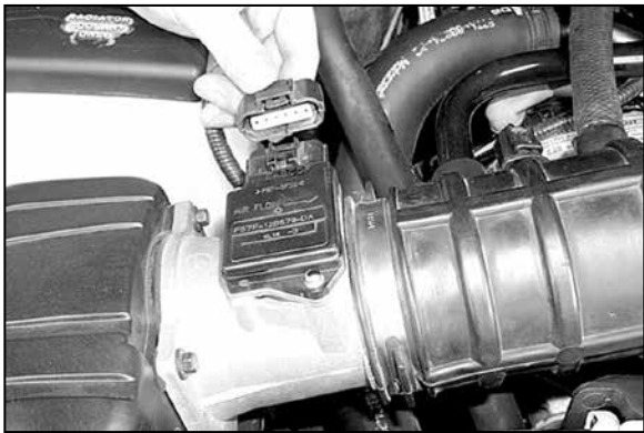
2. Disconnect the mass air sensor electrical connection.
