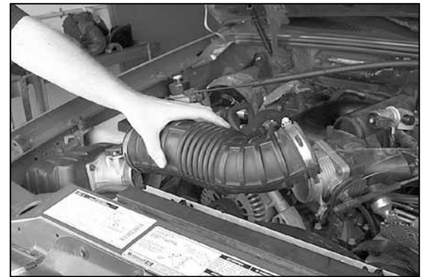
5. Loosen the hose clamps at the throttle body and the mass air sensor, then remove the air intake tube as shown
