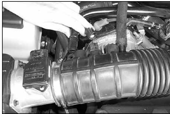
4. Remove the IAC vent, temp sensor and the CVC hose as shown
