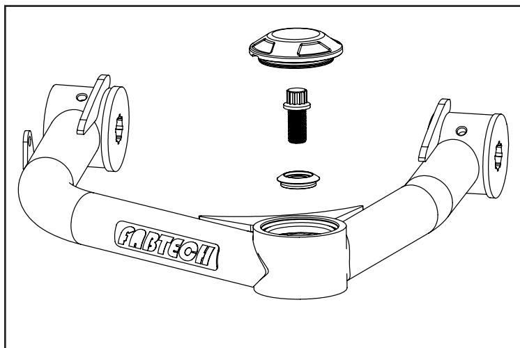
FIGURE 6 - STEP 10
