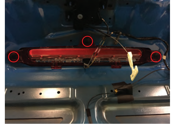
Step 3 Using a Phillips screw driver, remove the 3 plastic screw clips securing the factory brake light to the trunk. Then remove the brake light from the vehicle. Reinstall the Raxiom LED in reverse order.
