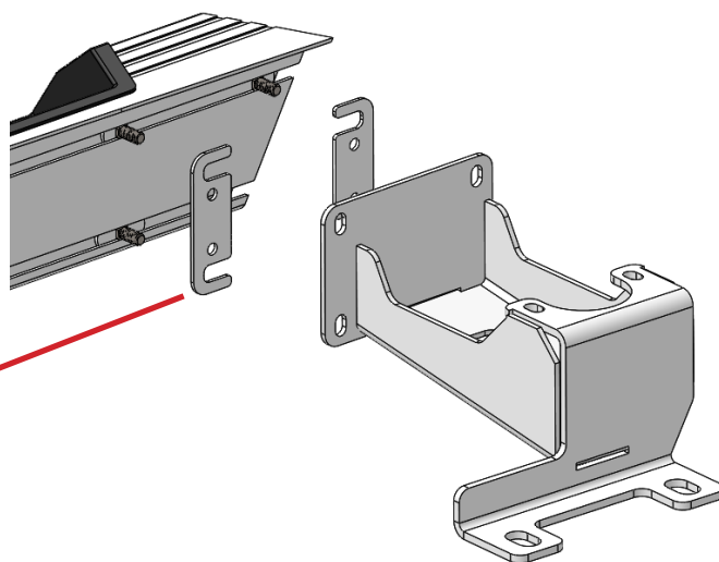
Shim Plate
