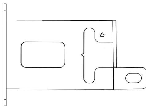
JT SLIDER CENTER MOUNT - PS 4JRS2060-12 (x1)
