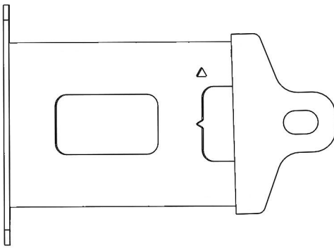
JT SLIDER FRONT MOUNT - PS 4JRS2060-01 (x1)
