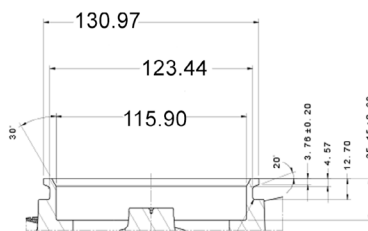
TURBINE OUTLET V-BAND
