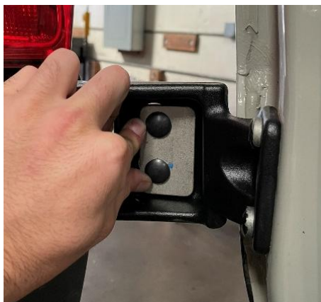
Figure 7: Lower Backing Plate Insertion
