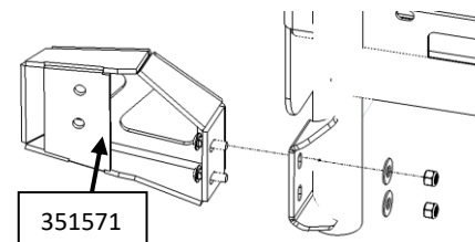
Figure 4: Heavy Duty Lower Hinge Bracket Installation
