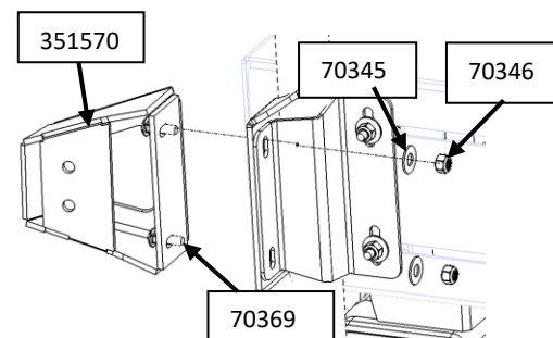
Figure 3: Heavy Duty Upper Hinge Bracket Installation
