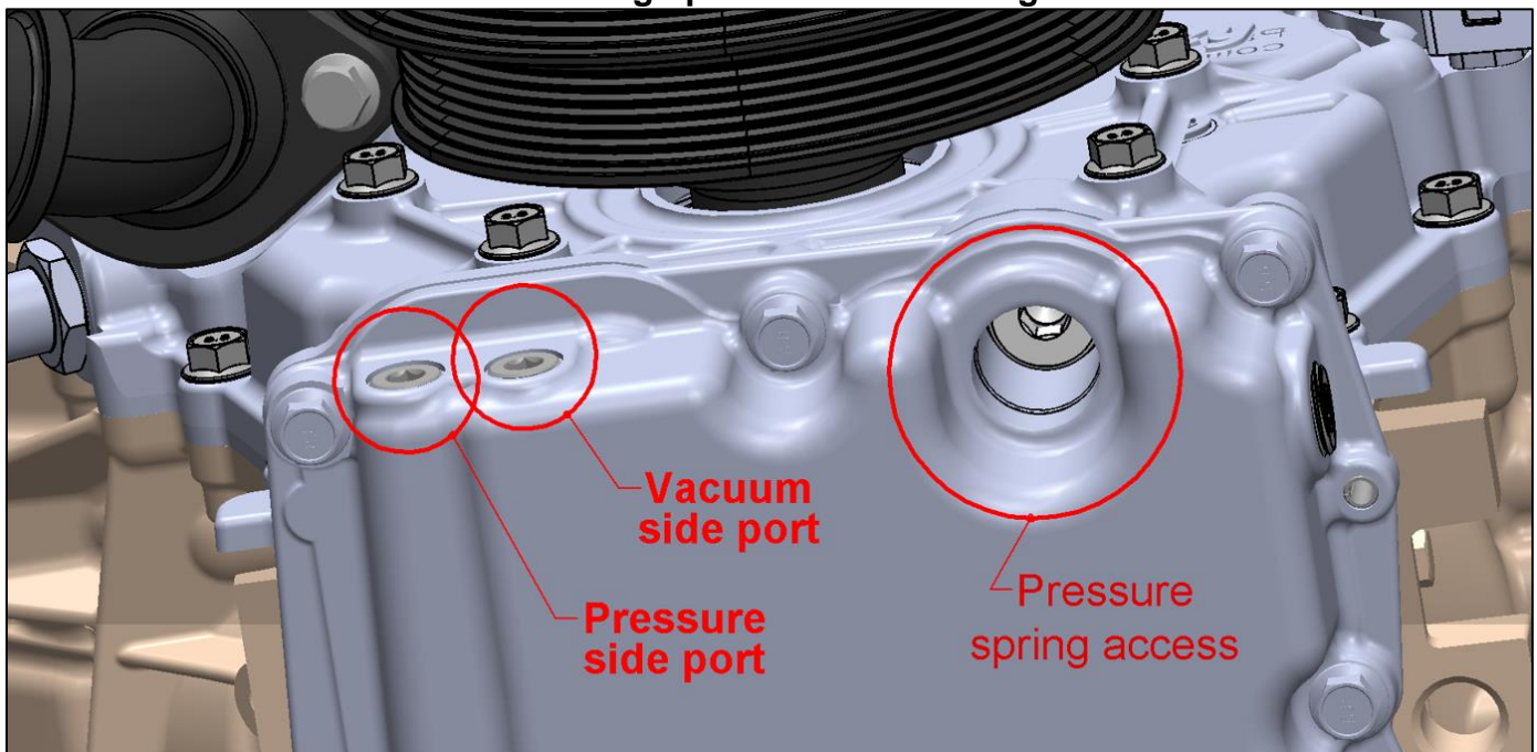
View looking up from under the engine.
