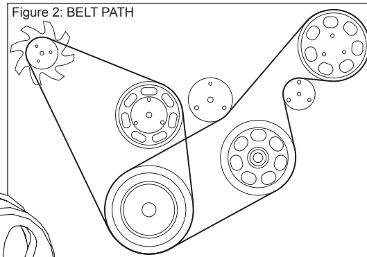
Figure 2: BELT PATH
