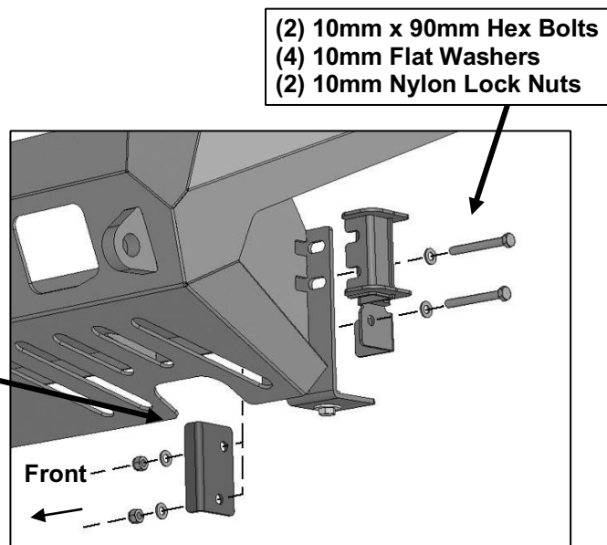
(Fig 16A) Slide the Outer Bumper Support Bracket under the (2) factory hex nuts. Attach Inner Support Bracket to frame and Outer Bracket (Driver/Left illustrated)
