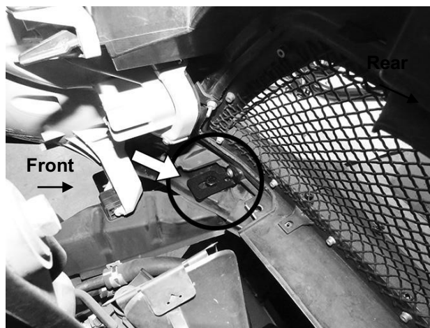
(Fig 21) Reinstall grille. Attach Grille Support Bracket to top of radiator core support (arrow). Reinstall plastic cover (also see Figure 2)
