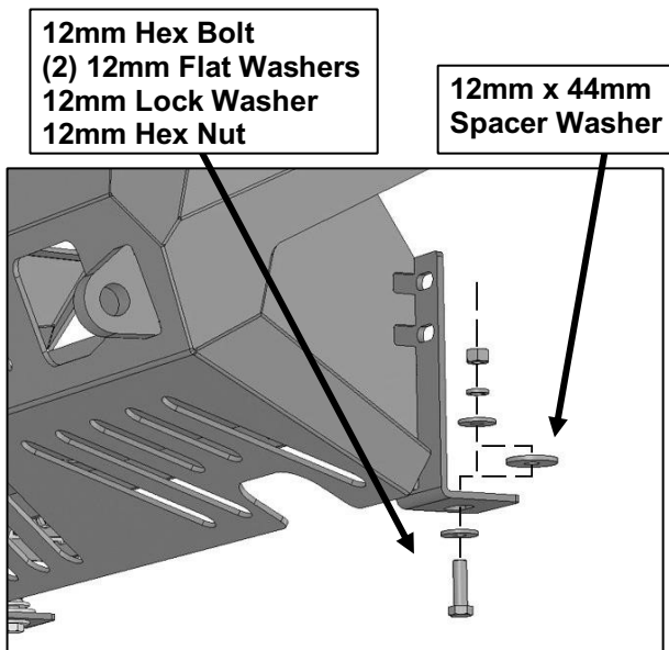
(Fig 14) Attach lower mounting tab on back of Bumper to bottom of crossmember. Insert 12mm x 44mm Spacer Washer between tab and crossmember as needed to level Bumper
