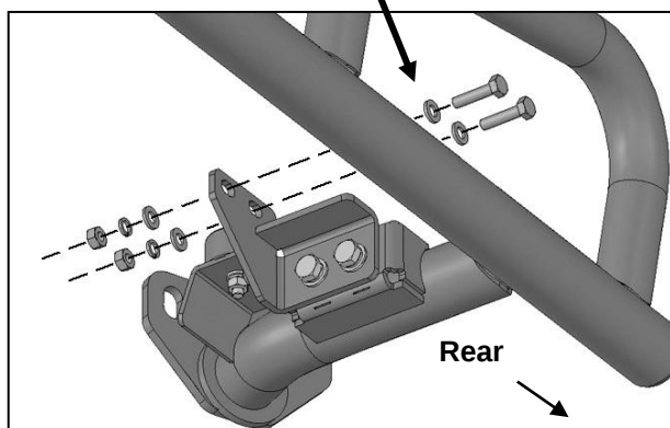
(Fig 26) Attach driver/left rear Support Bracket to outside of pinch weld, (stock height suspension installation illustrated)
