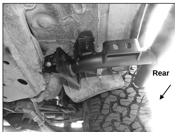
(Fig 18) Models with suspension lift "spacer," attach Adjustable Mounting Plate on end of Rocker Slider to rear Frame Bracket
