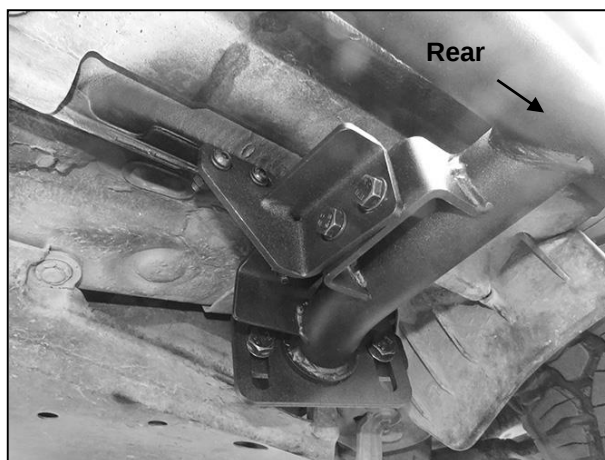
(Fig 27) Driver/left rear with spacer, (raised suspension), complete installation pictured
