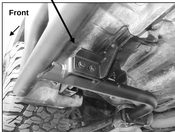
(Fig 25) Driver/left front complete installation
