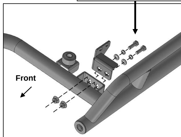
(Fig 19) Attach driver/left front Support Bracket to front end of Rocker Slider
