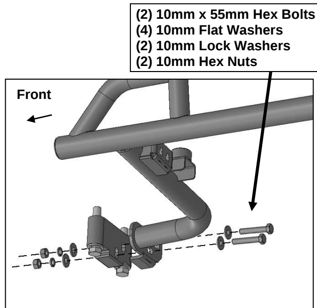
(Fig 14) Attach front of Rocker Slider to front Frame Mounting Bracket
