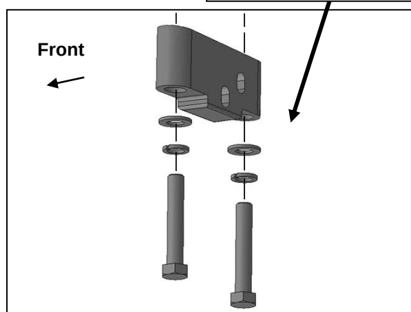
(Fig 2) Attach Front Frame Bracket to driver/left front mounting location (see Fig 1)
