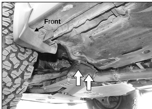
(Fig 1) Remove (2) factory hex bolts (arrows). Driver/left front pictured
