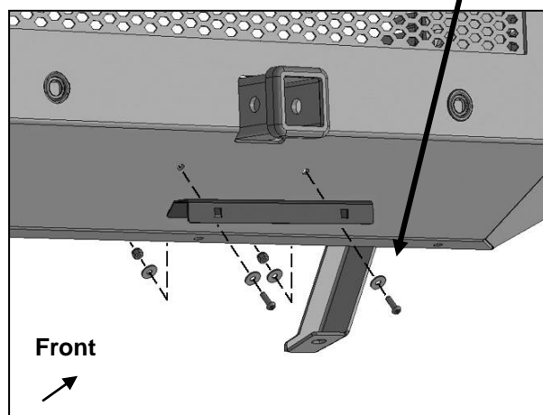
(Fig 20) Attach License Plate Bracket to Bumper before installing Skid Plate
