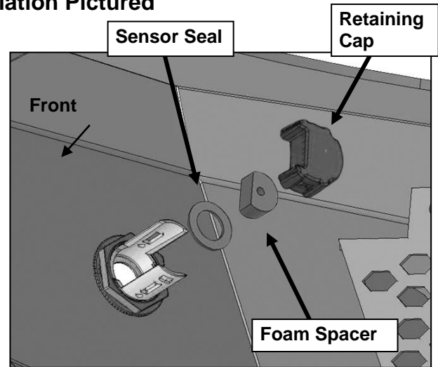
(Fig 10) Remove front seal from Sensor. Apply larger Foam Seal to sensor. Slide sensor into mount, insert Foam Spacer and Retaining Cap to lock sensor in mount
