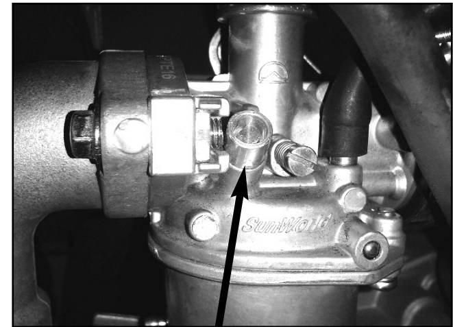
Air Screw location.
