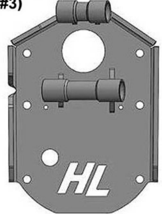
Rear Right Backing Plate (1ea) 117D-R
