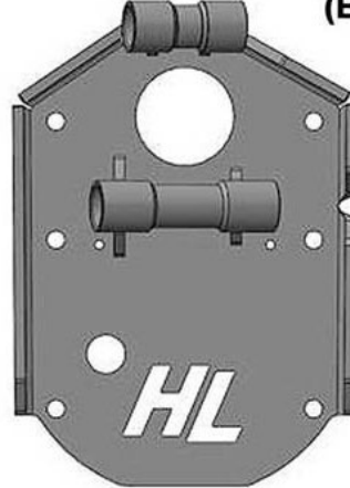
Rear Left Backing Plate (1ea) 117D-L
