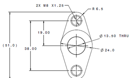
OIL OUTLET
