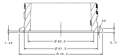
TURBINE INLET V-BAND CONNECTIONS
