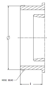
COMPRESSOR INLET HOSE CONNECTIONS Ø16.2 X 29.05
