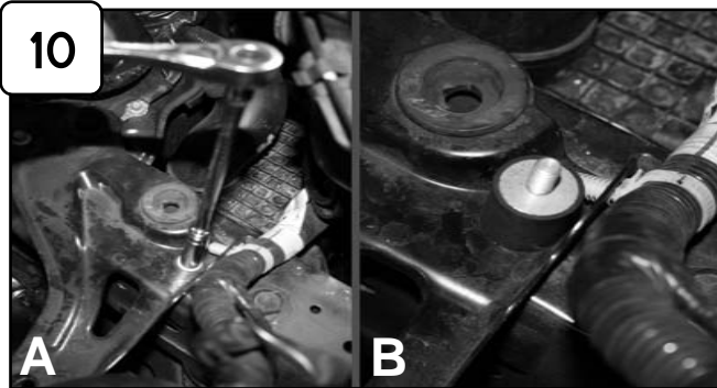
A) Loosen bolt next to grommet with 10mm socket or wrench. B) Replace using provided M8 isolation mount.
