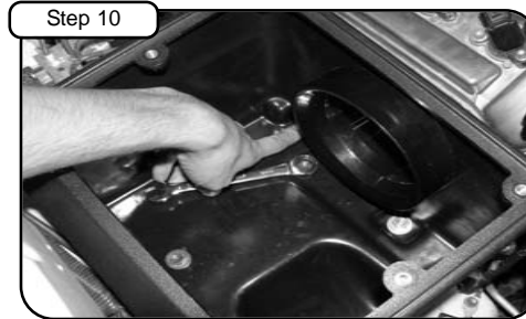
Place housing into vehicle and tighten using 12mm socket or wrench. With M8 nut and washer provided tighten down housing onto isolation mount with 13mm wrench.
